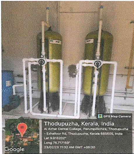
FINAL FILTER WITH CHLORINE DOSING
